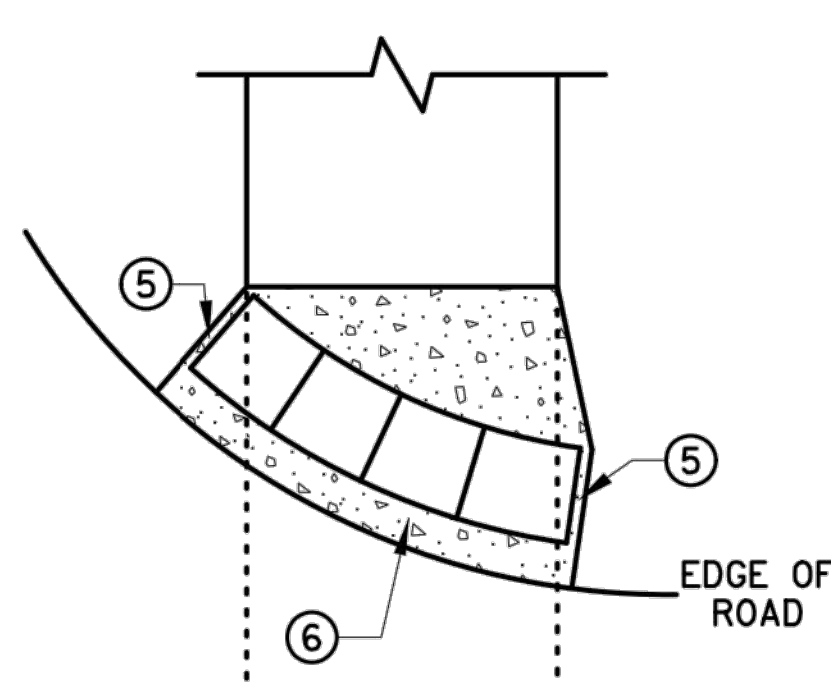
RADIAL DETECTABLE WARNING
