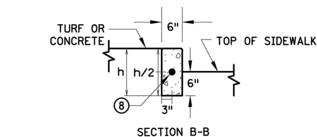
SECTION B-B
