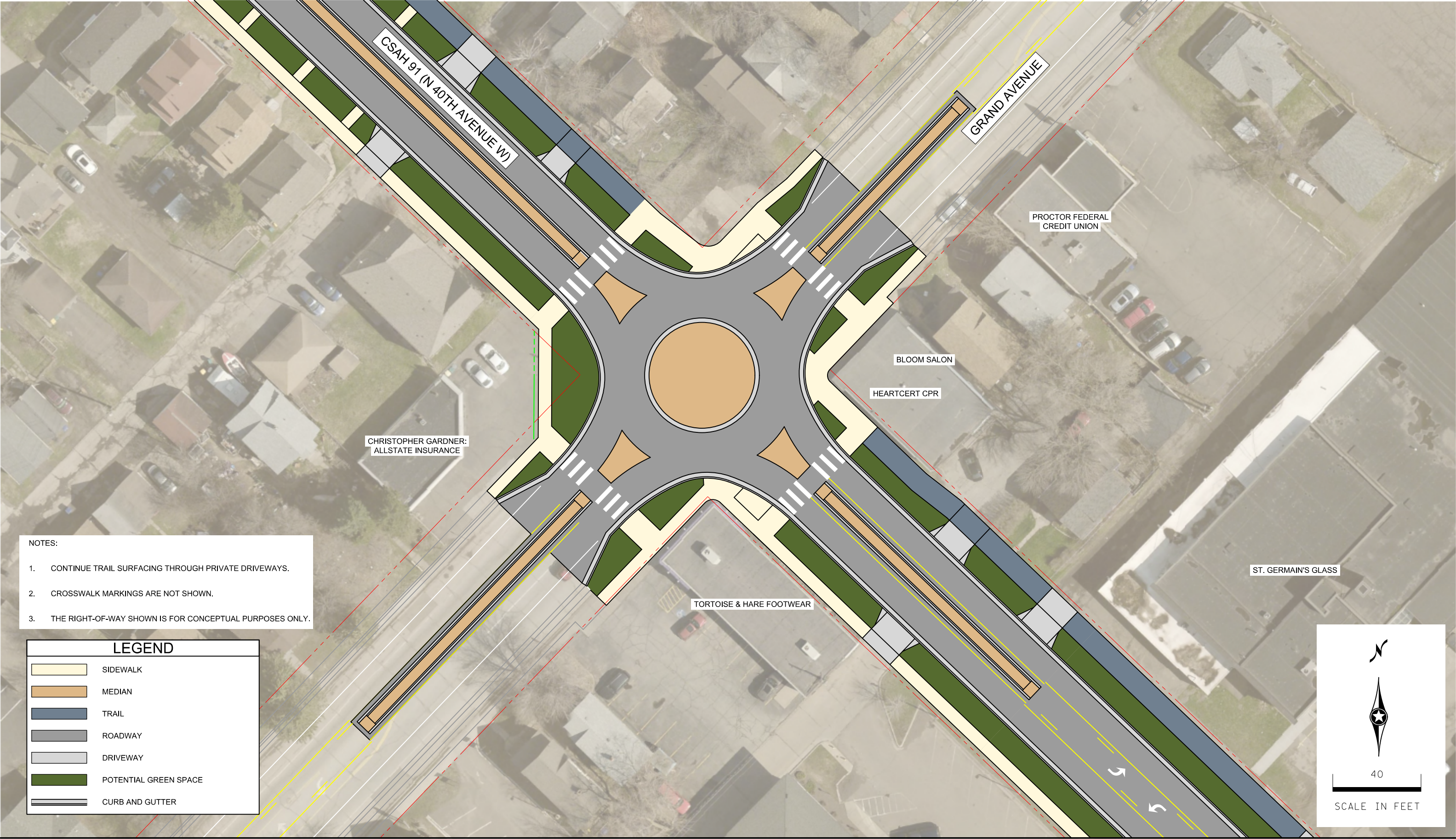
CSAH 91 (40th Ave W) and Grand Ave Intersection Control Evaluation
