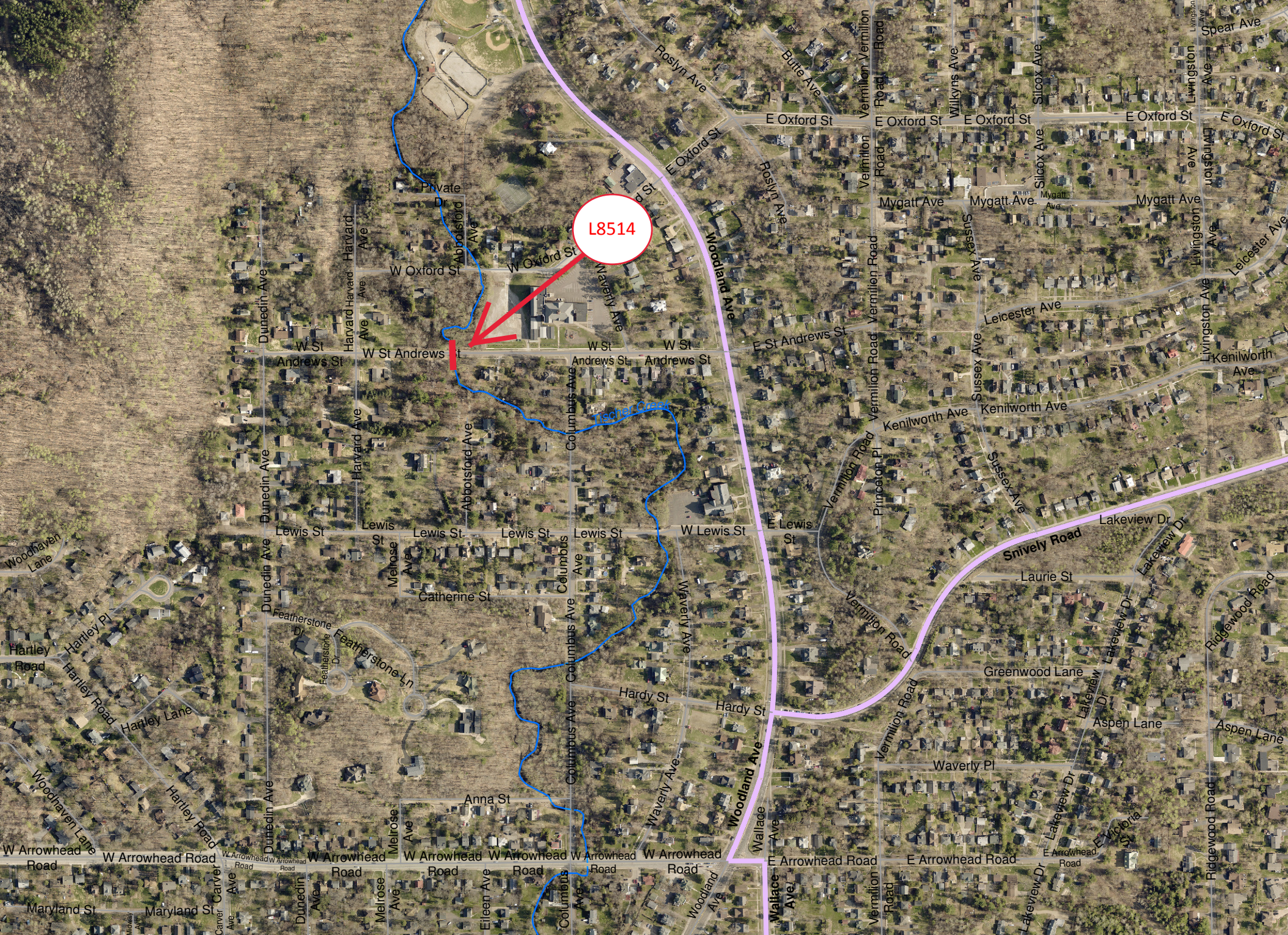
REPLACE BRIDGE L8514 ST. ANDREWS STREET OVER TISCHER CREEK PROJECT NO. 1861
