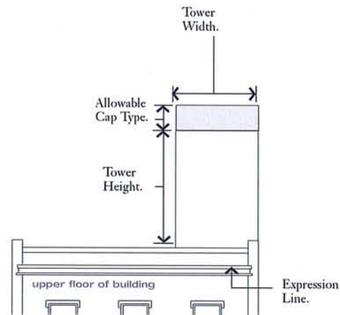
Figure 50-22.4-D: Tower
