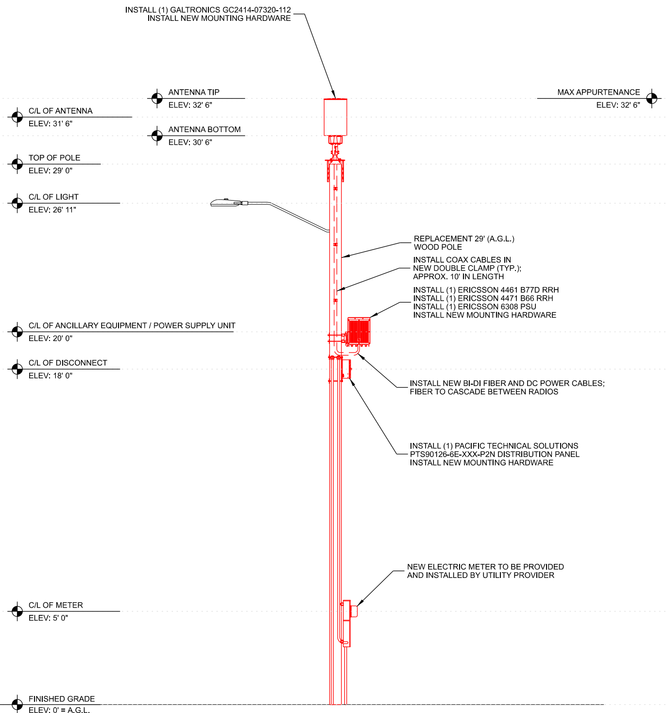
B PROPOSED ELEVATION
