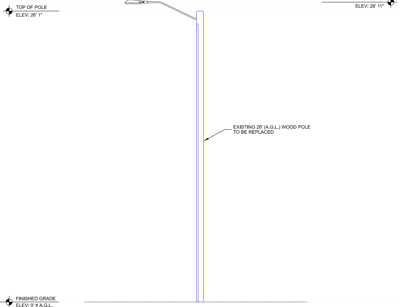
A EXISTING ELEVATION
