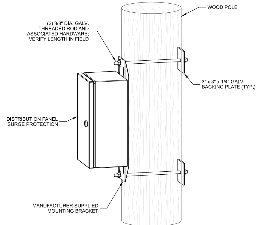
C DISTRIBUTION PANEL / SURGE PROTECTION MOUNT
