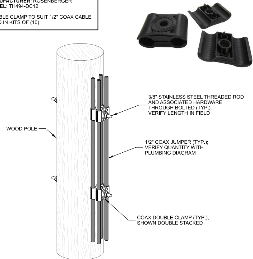
F COAX DOUBLE CLAMP ANT.13858
